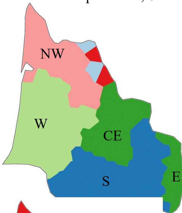
Complete link, 6
